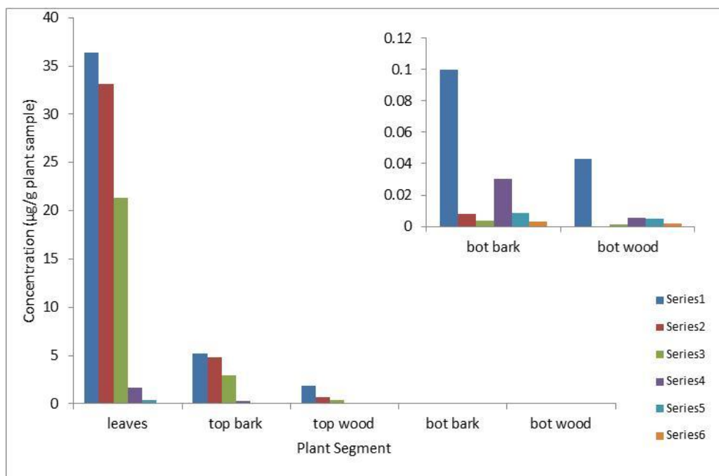
Figure 2-8. Distribution of PCBs throughout the plant in the Dead Poplar Control measured in µg/g of plant sample for Exposure 2
